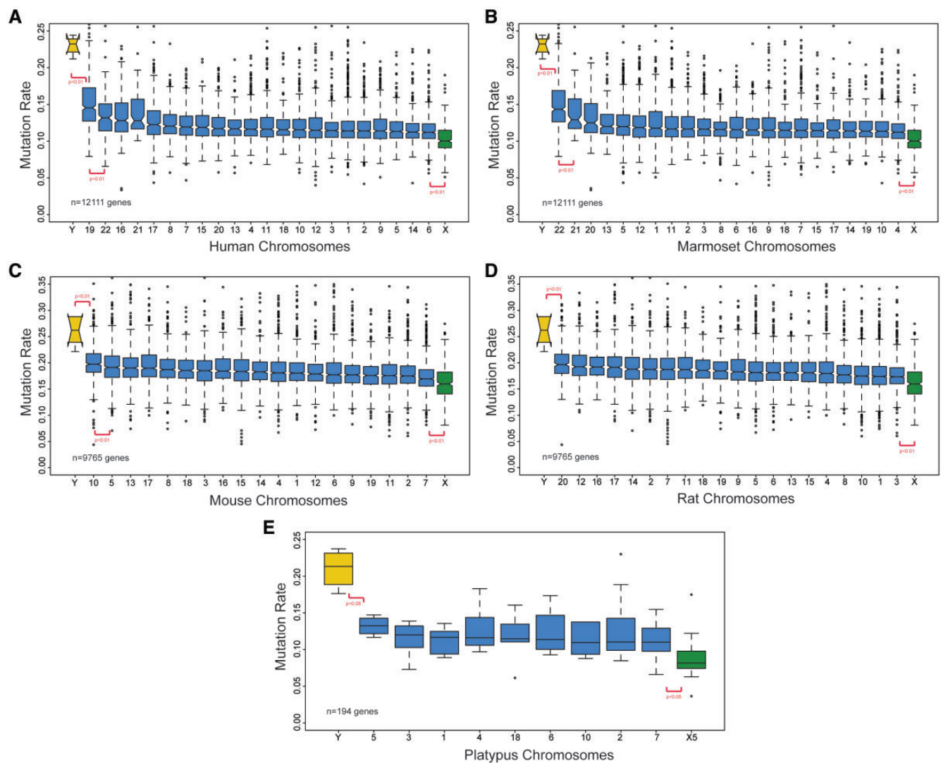
FIG. 1. —Substitution rates across all chromosomes in monotremes and control species. (a, b) Substitution rates from the human–marmoset comparisons, sorted according to the human homologous chromosomes (a) or the marmoset homologous chromosomes (b). (c, d) Substitution rates from the mouse–rat comparisons, sorted according to the mouse homologous chromosomes (c) or the rat homologous chromosomes (d). (e) Substitution rates from the platypus–echidna comparisons, sorted according to the platypus chromosomes. Data for the echidna could not be plotted because there is no reference genome for this species. Chromosomes are sorted according to their median substitution rate in descending order, from left to right. P -values were obtained by applying the Benjamini–Hochberg-corrected Welch Two Sample t -test. See supplementary table 7, Supplementary Material online for correspondence between human–marmoset and mouse–rat homologous chromosomes.
