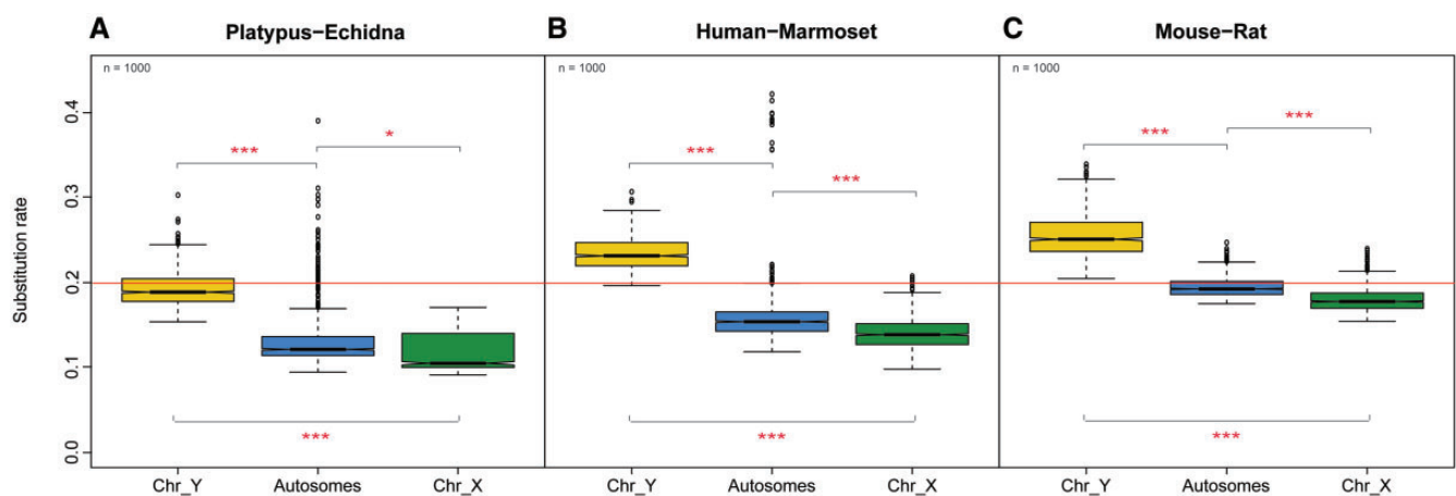
Fig. 2. —Distribution of chromosomal substitution rates in monotremes and control species. Distributions of chromosomal substitution rates for Y, X, and autosomes in monotremes (a), primates (b), and rodents (c) obtained from 1,000 bootstrap rounds. Significance of the Welch Two Sample t -test Benjamini–Hochberg-corrected P values are as follows: *** P < 0.001, * P < 0.05. Error bars, maximum and minimum values, excluding outliers. The red line at value 0.2 serves as visual aid.
